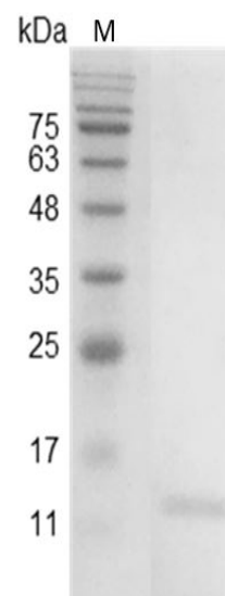
SDS-PAGE analysis of recombinant mouse IL-9
